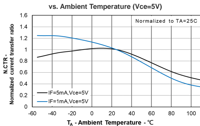
Figure 11. Normalized Current Transfer Ratio
